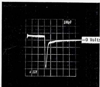
Fig. 0E: Output voltage waveform of WQ-10C at the relative intensity setting = 3 and its basic electrical parameters.
